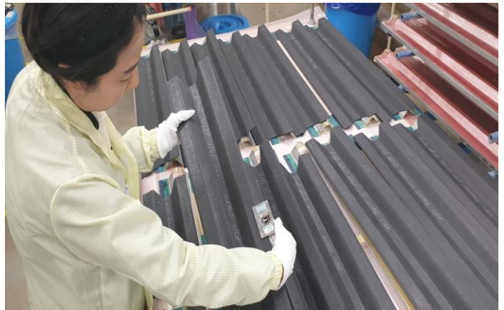
787 AFTBODY STRINGER WIDTH EDGE INSPECTION
