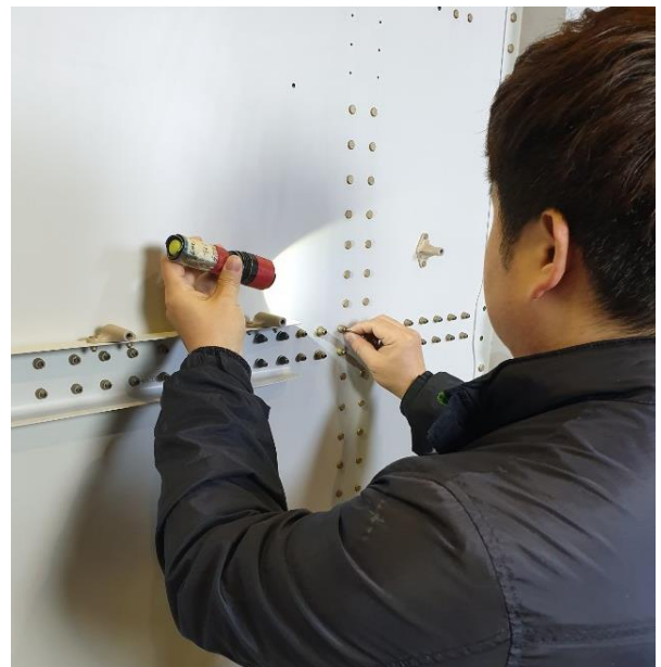
787 AWWB HI-LOK BOLT INSPECTION
